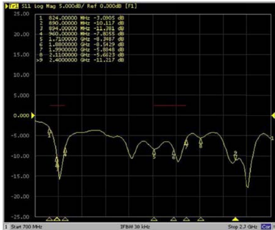
Log Mag Quad Band
