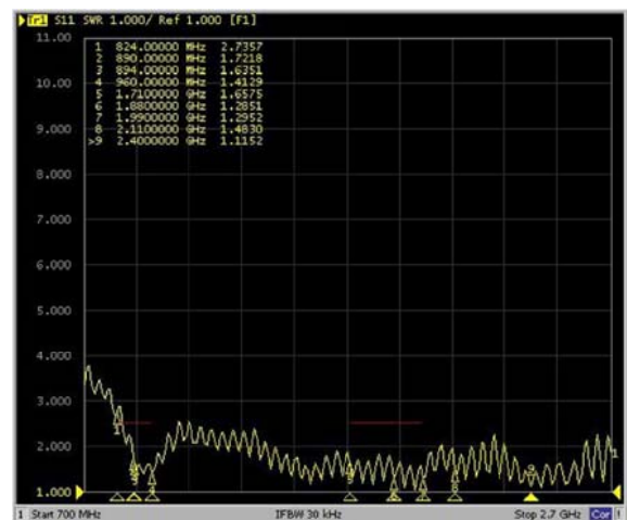
VSWR Quad Band
