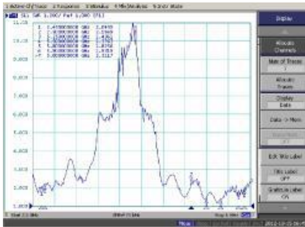
Bluetooth / Wifi V.S.W.R. Curve
