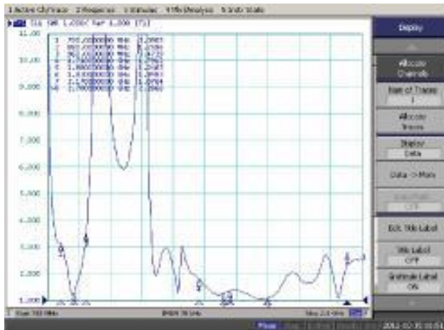
LTE V.S.W.R. Curve
