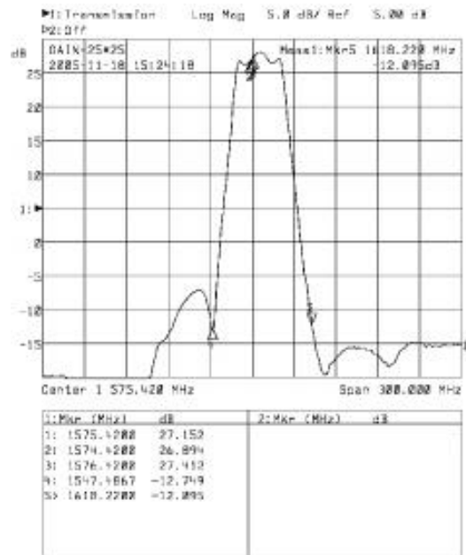
GPS V.S.W.R. Curve
